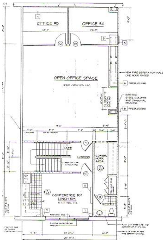
SECOND FLOOR PLAN 3/16 = 1'-0"
