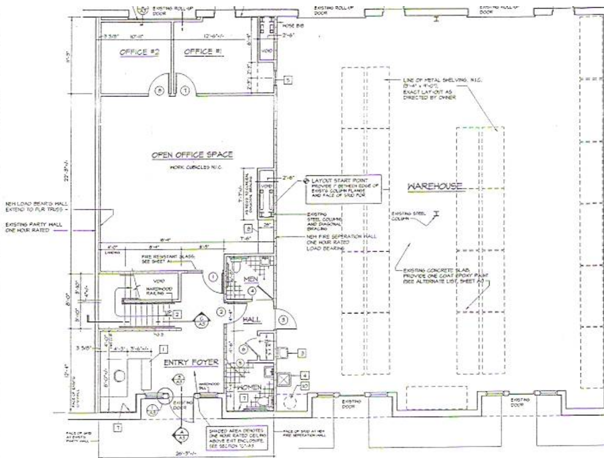
FIRST FLOOR PLAN 3/16 = 1'-0"
